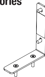
IDI-14T0108 Adapter ID14 to IDS108
