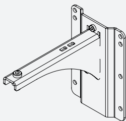
VNI-WM200 Wall mount 200 mm
