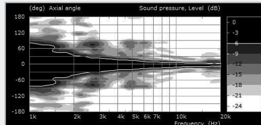
STM HF waveguide coverage versus theoretical 5° curved linear source.
