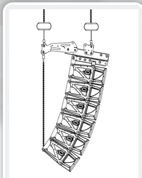
Array angles realised after lifting
