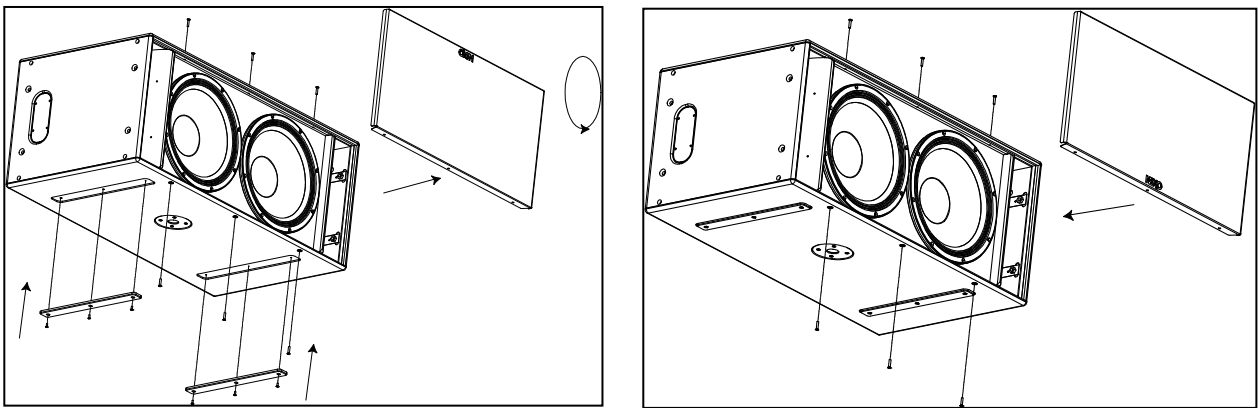
CONFIGURING RS15 AS LEFT
