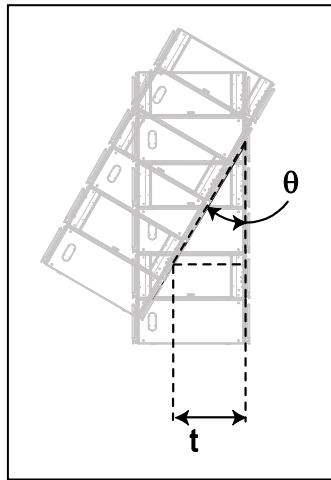
GROUP OF 3 RS15S STEERING
