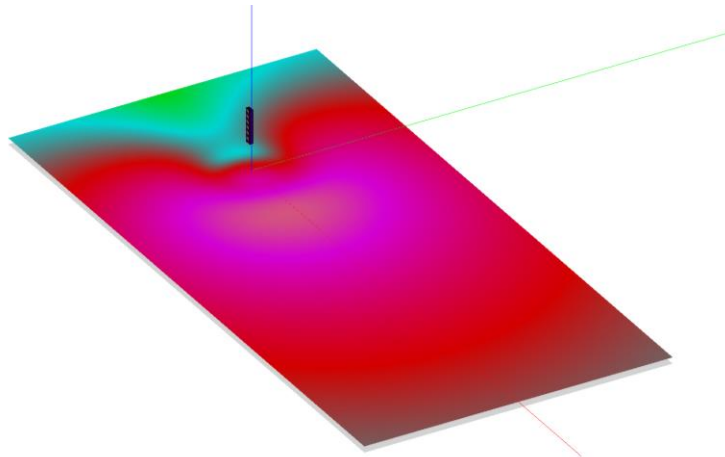
10 RS18 CLUSTER OVER 75M/200FT, STEERED 15° DOWN
