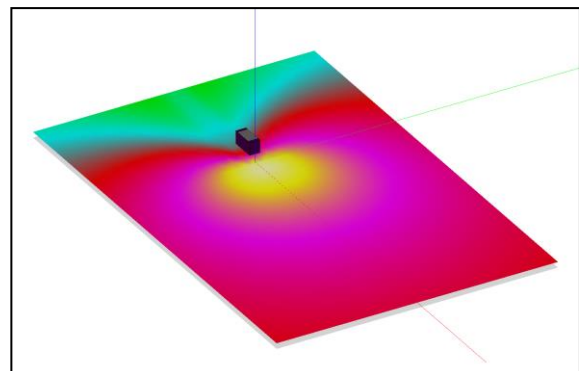
VERTICAL COVERAGE IN DIRECTIONAL MODE
