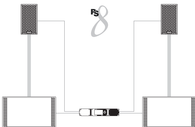
NXAMP4X1 MK2 powering 1 X PS8 and 1 X LS400 Sub per side
